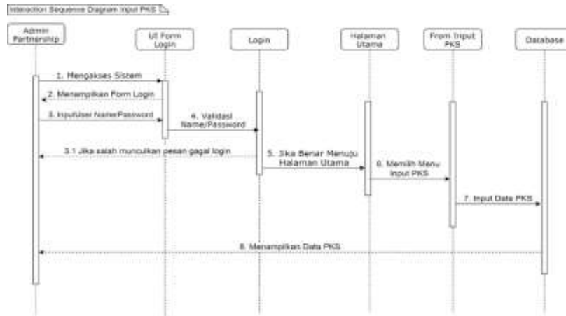
Gambar 5. Sequence Diagram Input Data Perjanjian Kerja Sama
