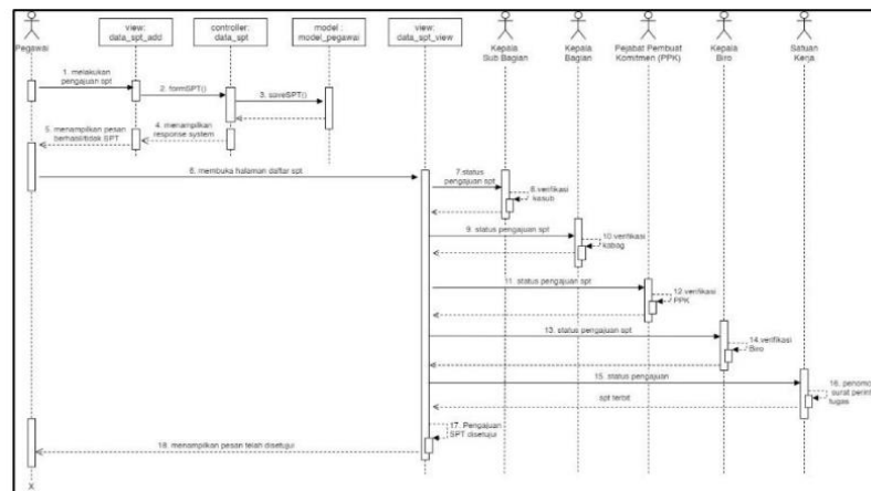
Gambar 4. Sequence Diagram
