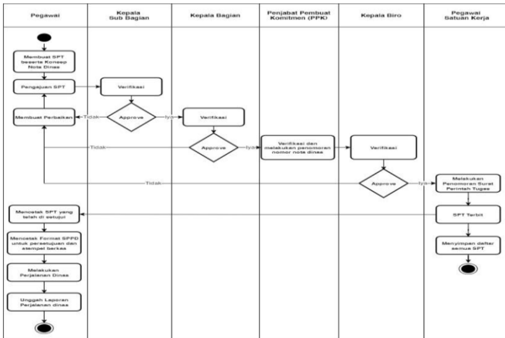
Gambar 3. Activity Diagram Menu
