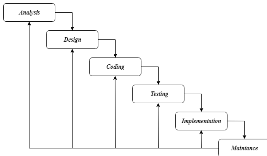
Gambar 1. Waterfall Model
