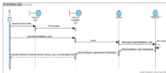
Gambar 4. Sequence Diagram
